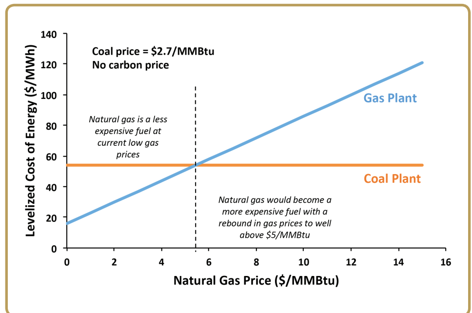
Figure 1: Effect of natural gas price on economics of coal- vs. gas-fired power
