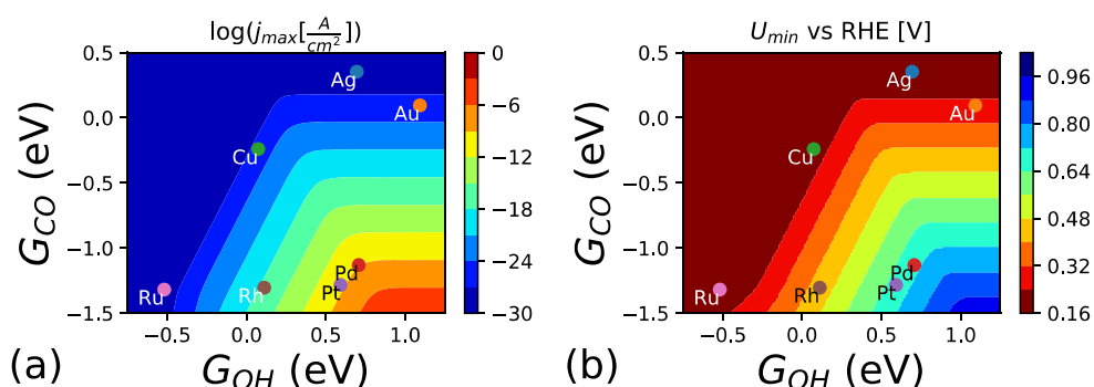
Figure 7. Contour plots for methane oxidation activity as a function of the free energy of adsorption of CO (relative to CO(g)) and OH (relative to H 2 O(l)/H 2 (g)). (a) The maximum attainable current density for electrochemical methane oxidation at ambient conditions for several metals and (b) the minimum electrochemical potential (V vs RHE) required to achieve the maximum current density.
