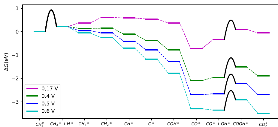
Figure 3. Free energy diagram at 300 K and 1 bar gas-phase pressures for the complete electrochemical oxidation of methane to carbon dioxide on Pt(211) at four representative electrode potentials: 0.17 (the equilibrium potential), 0.40, 0.50, and 0.60 V vs RHE. The x -axis labels denote the relevant surface species for each step.
