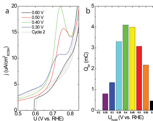
Figure 4. (a) Electrode potential dependence of oxidation feature in 0.5 M perchloric acid after holding the electrode potential constant for 30 min (ECSA \sim 220 cm 2 , scan rate 50 mV/s). (b) Total integrated stripping charge for the different electrode hold potentials.
