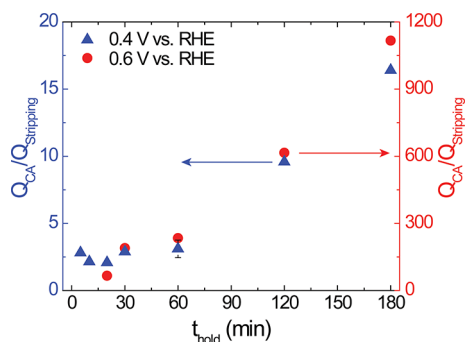
Figure 5. Ratio of charge transferred during the electrode potential hold ( Q_{CA} ) to the stripping feature ( Q_{Stripping} ) at an electrode hold potential of 0.4 V vs RHE (blue, left axis) and 0.6 V vs RHE (red, right axis) as a function of electrode potential hold length. Slopes were fit to the last three data points for each potential. No distinguishable stripping feature was observed at 5 and 10 min electrode potential holds at 0.6 V vs RHE.
