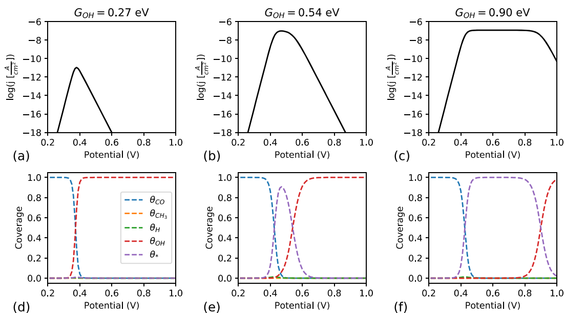
Figure 6. Methane oxidation kinetics for different values of \text{OH}^* binding with P_{\text{CH}_4} = 1 bar and P_{\text{CO}_2} = 1 mbar. Panels (a–c) contain log current densities for G_{\text{OH}} = 0.27, 0.54, and 0.9 eV, respectively, as a function of electrochemical potential (V vs RHE) assuming a site density of 10^{15} sites/ \text{cm}^2 and \sim 6.2\% of the ECSA being active for methane oxidation (as in SI section 10); panels (d–f) contain coverages of key intermediates as a function of potential (V vs RHE) for G_{\text{OH}} = 0.27, 0.54, and 0.9 eV, respectively.
